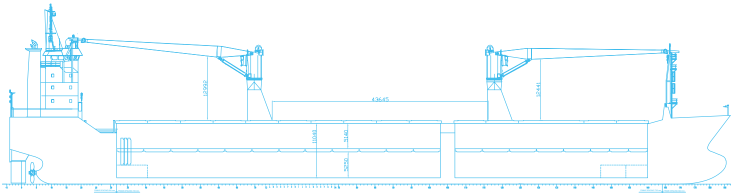
Side view
